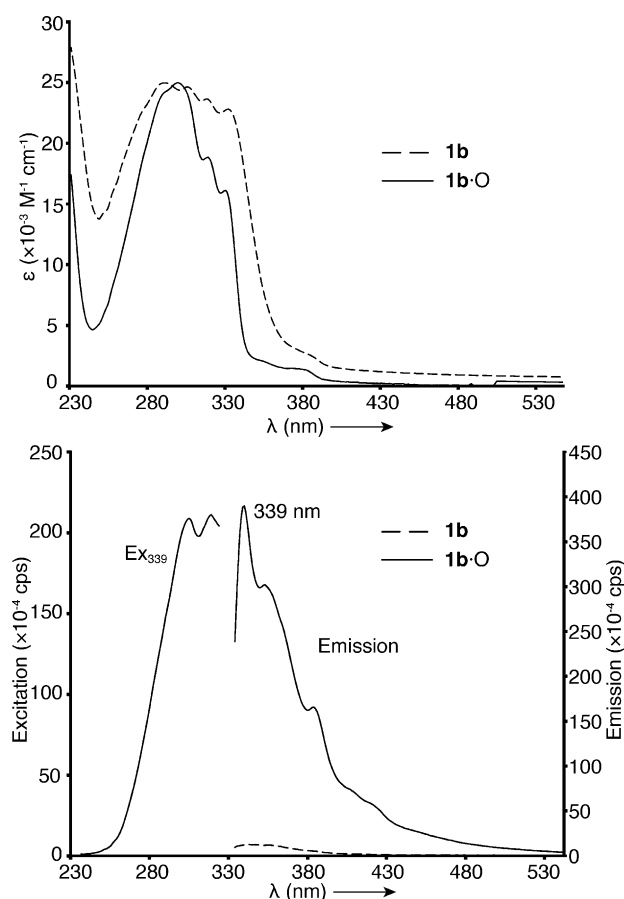
Figure 4. UV/Vis absorption spectra (top); emission and excitation spectra (bottom) of 1b and 1b-O in THF solution ( 10^{-5} M). The excitation spectrum labelled Ex 339 was recorded for the emission maxima at 339 nm, respectively. The emission spectra were recorded with excitation wavelength 318 nm. The abbreviation cps stands for counts per second.
