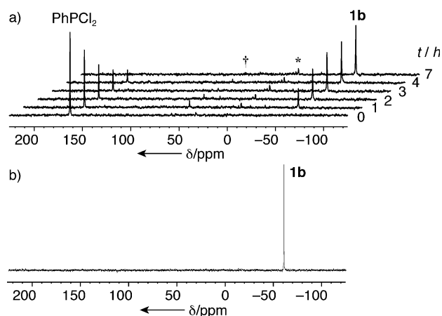
Figure 1. a) Selected ^{31}\text{P} NMR spectra (121.5 MHz, toluene, 358 K) showing: the progress of the polymerization of \text{PhPCl}_2 and 1,4-diethynyl-2,5- n -diethylbenzene using \text{Ni}(\text{acac})_2 (5 mol %) as catalyst and \text{NEt}_3 (6 equiv) as base (trial 1). The measurement times are given in hours. \dagger indicates signals assigned to -\text{P}(\text{Ph})\text{Cl} moieties. We speculate that the signals marked with * result from hydrolysis of \text{PhPCl}_2 by traces of water found in the nickel(II) catalyst. b) ^{31}\text{P} NMR spectrum (121.5 MHz, \text{CDCl}_3 , 358 K) of isolated polymer 1b after precipitation.
