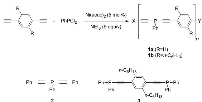
Scheme 1. Synthetic procedure to poly( p -phenylenediethynylene phosphane)s (PPYPs) 1a and 1b . Analogous procedures are used to prepare model compounds 2 and 3 . For each model and polymer, the corresponding phosphane oxide has also been prepared and fully characterized (e.g. 1b -O, 2 -O and 3 -O).
