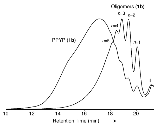
Figure 2. Gel permeation chromatography (GPC) traces of PPYP ( 1b ) [trial 1: M_w = 10,000 Da; \text{PDI} = 2.0 , vs. polystyrene standards] and the methanol-soluble fraction containing oligomers of 1b ( n = 1-5 are resolved; \text{X} = \text{H}-\text{C}\equiv\text{C}- ; \text{Y} = -\text{C}_6\text{H}_2\text{R}_2-\text{C}\equiv\text{C}-\text{H} ). The assignments are tentative. [\dagger] assigned to monomer 1,4-diethynyl-2,5-di- n -hexylbenzene by comparison to the GPC trace of an authentic sample.
