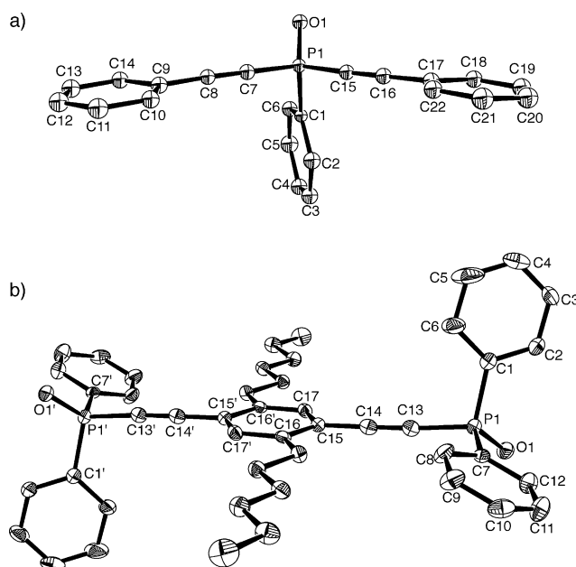
Figure 3. Molecular structures of 2-O (a) and 3-O (b) (50% probability ellipsoids). Hydrogen atoms are omitted for clarity. Selected distances (Å) and angles (°): 2-O (a): P1-O1 1.481(2), P1-C1 1.793(3), P1-C7 1.751(3), P1-C15 1.750(3), C7-C8 1.201(4), C8-C9 1.443(4), C15-C16 1.204(4), C16-C17 1.439(4); C1-P1-C7 105.57(13), C1-P1-C15 105.30(13), C1-P1-O1 113.22(13), C7-P1-O1 115.08(12), C15-P1-O1 112.64(12), P1-C7-C8 173.6(3), C7-C8-C9 178.0(3), P1-C15-C16 173.4(3), C15-C16-C17 178.1(3); 3-O (b): P1-O1 1.480(2), P1-C1 1.802(3), P1-C7 1.797(3), P1-C13 1.746(3), C13-C14 1.196(4), C14-C15 1.441(4); C1-P1-C7 107.3(1), C1-P1-C13 104.6(1), C1-P1-O1 112.5(1), C7-P1-O1 111.1(1), C13-P1-O1 116.0(1), C7-P1-C13 104.6(1), P1-C13-C14 176.5(3), C13-C14-C15 178.7(3). Angles between planes (°): 2-O (a): C9-C14 and C17-C22 9.1, C1-C6 and C9-C14 79.9, C1-C6 and C17-C22 88.5; 3-O (b): C15-C17' and C7-C12 23.6, C15-C17' and C1-C6 82.3.
